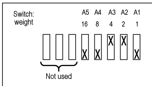
Figure 3: GPIB DIP switch on rear panel
