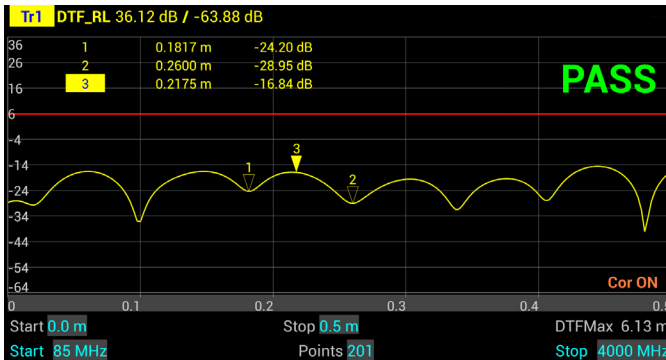
Figure 18 Active Marker
