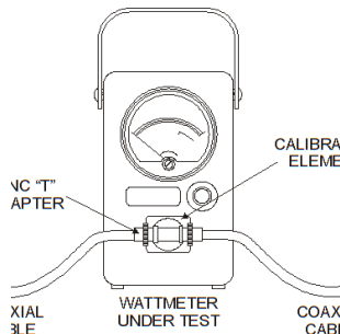
Figure 11 Calibration Setup
