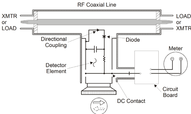
Figure 2 Schematic
